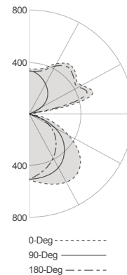
PHOTOMETRICS
