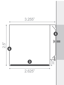
CROSS-SECTION
